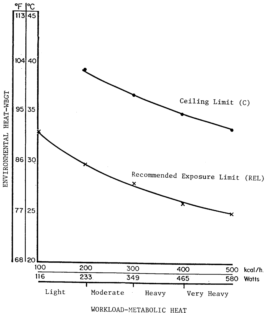
Figure 1. Recommended Heat-Stress Exposure Limits for Acclimatized Workers
